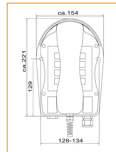
Dimensioned drawing: dA24/ZB
